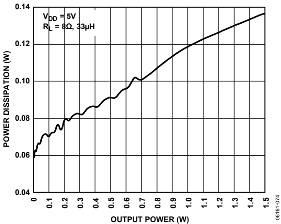
Figure 29. Power Dissipation vs. Output Power into 8Ω at V_{DD} = 5.0V
