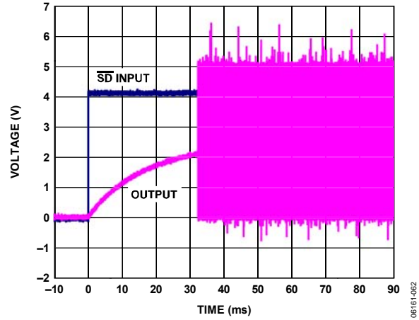
Figure 41. Turn-On Response
