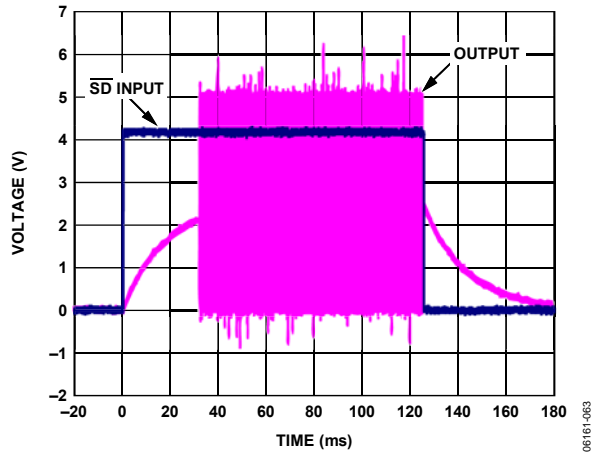
Figure 42. Turn-Off Response
